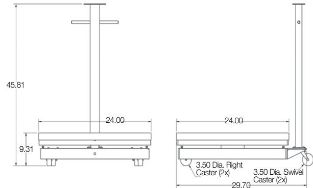
Caster Model
