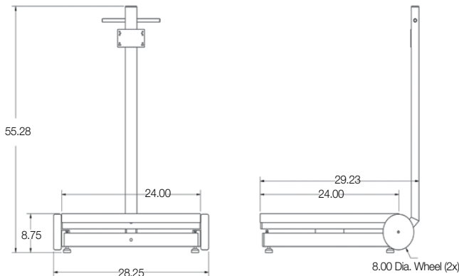
Wheel Model
